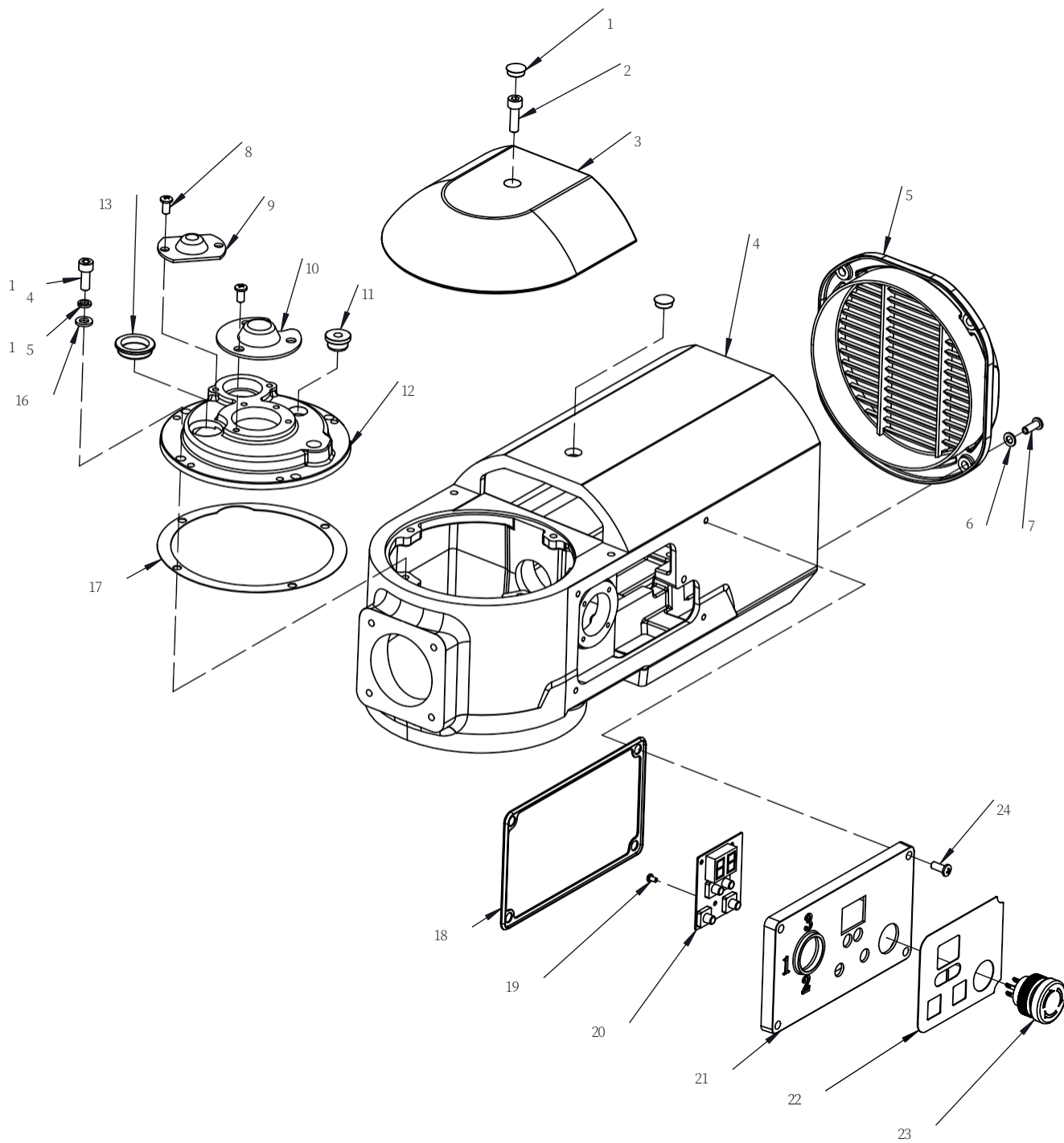
EC10 4-function gearbox complete set
